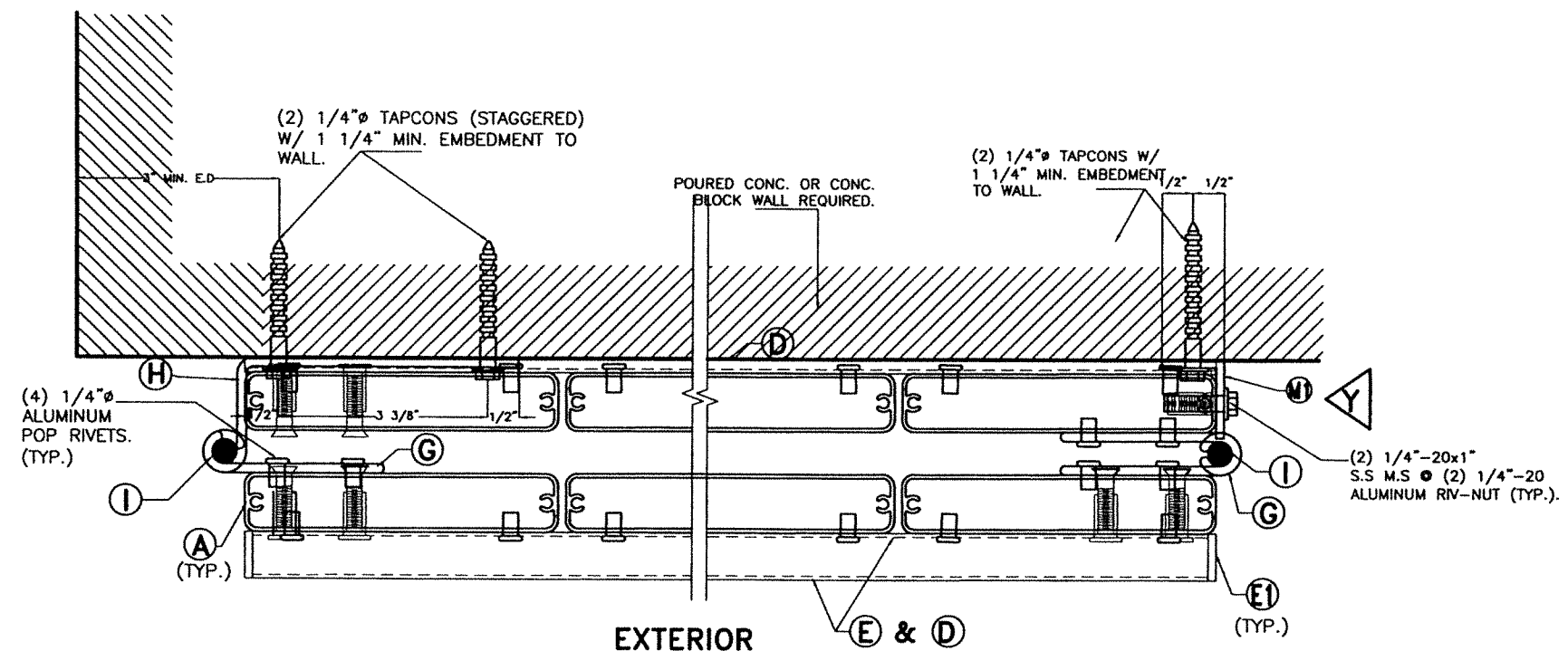
DETAIL 4 (NON HURRICANE POSITION)
