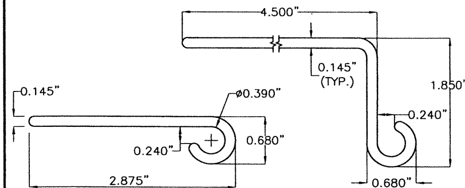
H SINGLE HINGE FOR POURED CONCRETE OR CONCRETE BLOCK WALL 6063-T6 Alum. ALLOY 2" LONG.
