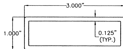
L1 STORM BAR TYPE 1 6063-T6 Alum. ALLOY
