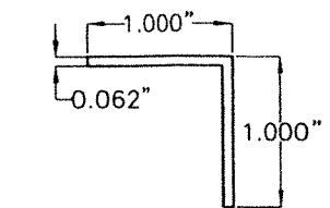
F TOP & BOTTOM CAP ANGLE 6063-T6 Alum. ALLOY
