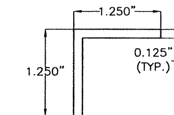
M1 NON HURRICANE BRACKET ANGLE 6063-T6 Alum. ALLOY 2 1/8" LONG.
