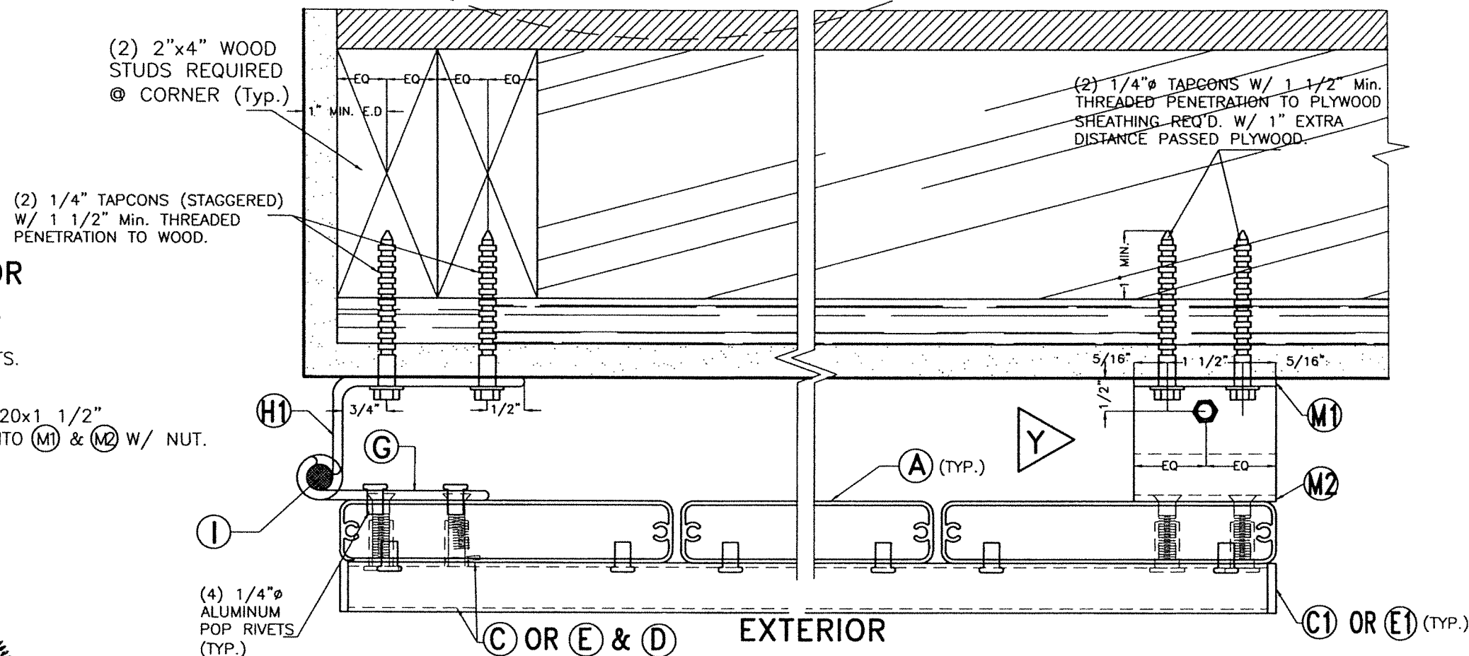
DETAIL 3 (NON HURRICANE POSITION) SCALE: 1/2"=1"
