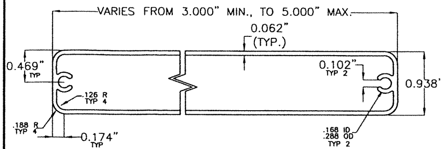
A 0.938"xVARIES SLAT (BOARD) 6063-T6 Alum. ALLOY
